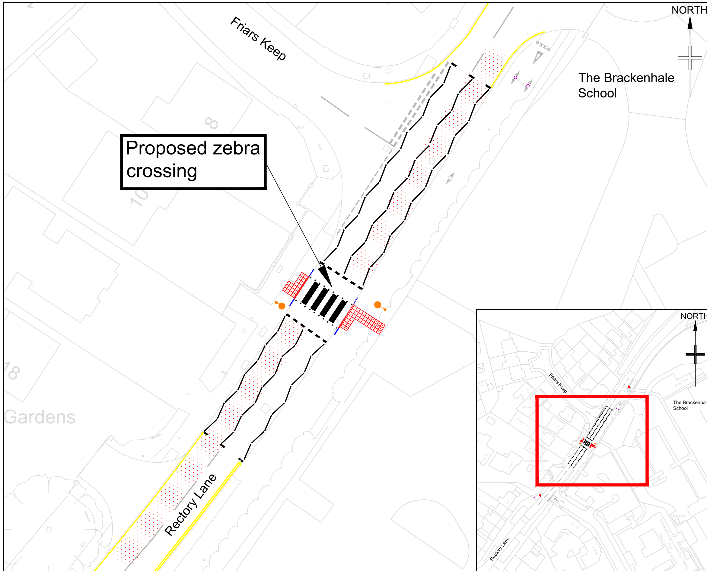
Construction Layout Plan Scale - 1:250
